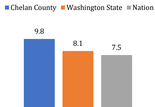
Exhibit 35: Air Pollution – Particulate Matter
